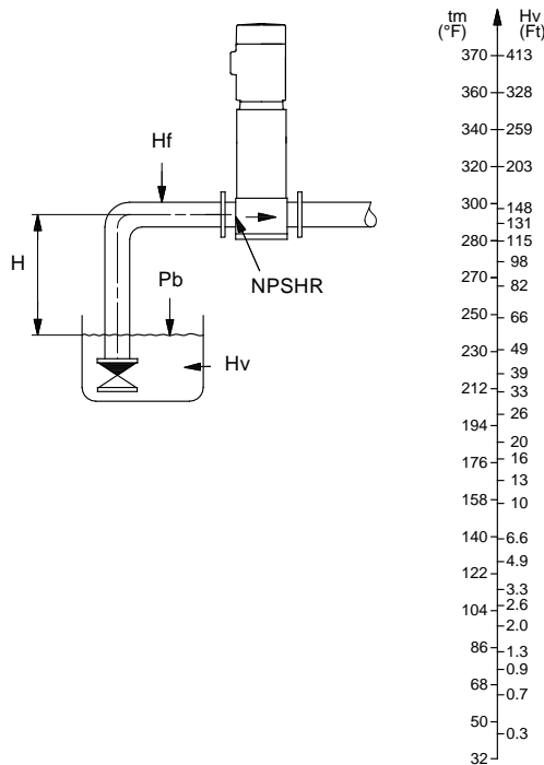
Fig. 26 Minimum inlet pressure - NPSHR
